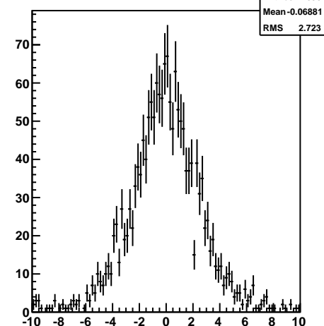
pull py of daughter2, chi2prob &lt; 0.02
