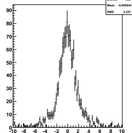
pull v0vertex Y, chi2prob &lt; 0.02
