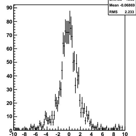
pull v0vertex X, chi2prob &lt; 0.02
