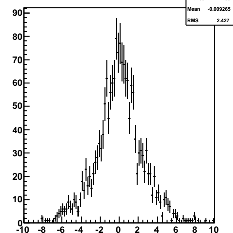
pull pz of daughter2, chi2prob &lt; 0.02
