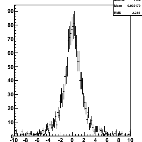
pull v0vertex Z, chi2prob &lt; 0.02
