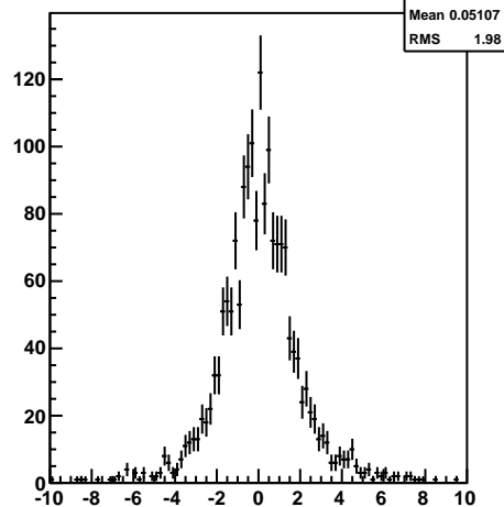
pull py of daughter1, chi2prob &lt; 0.02
