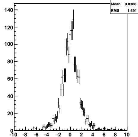
pull pz of daughter1, chi2prob &lt; 0.02
