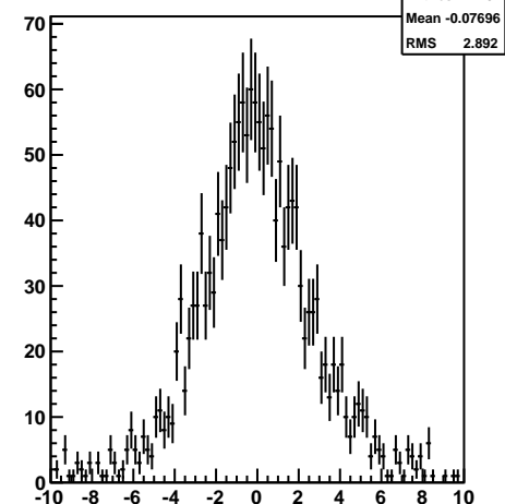
pull px of daughter2, chi2prob &lt; 0.02
