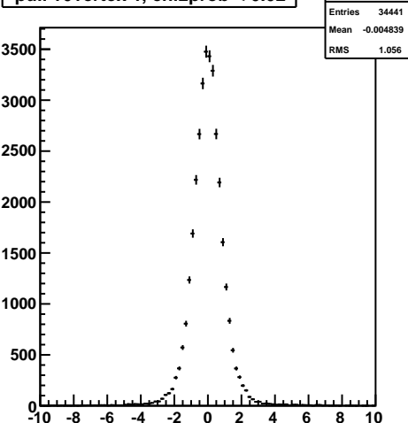
pull v0vertex Y, chi2prob < 0.02
