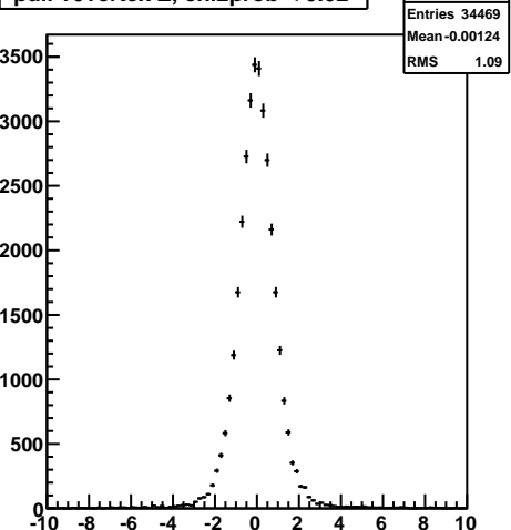
pull v0vertex Z, chi2prob < 0.02
