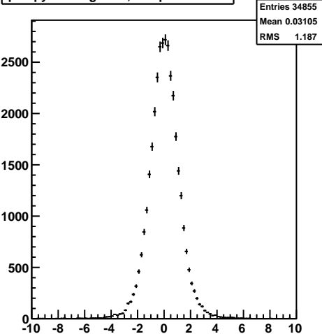
pull py of daughter1, chi2prob < 0.02
