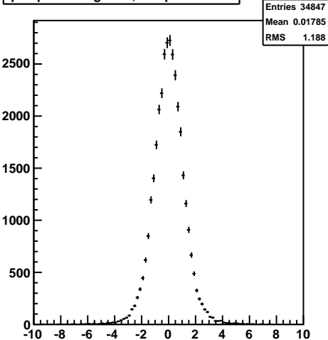
pull px of daughter1, chi2prob < 0.02
