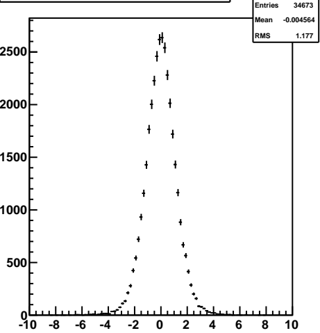
pull pz of daughter2, chi2prob < 0.02
