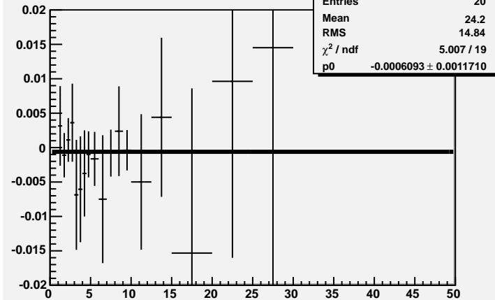
rates K0s
