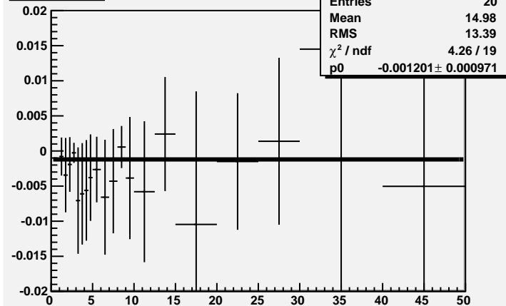
sumpt K0s
