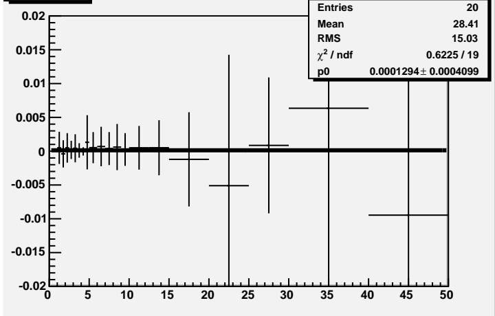
rates K0s
