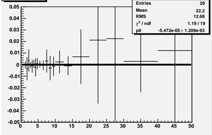
rates LA,AL
