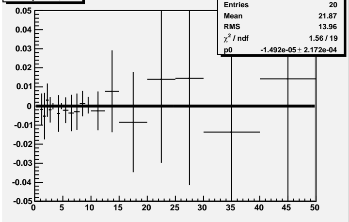
sumpt LA,AL
