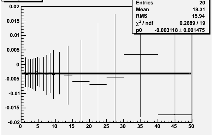
sumpt K0s
