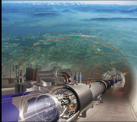
proton collisions
