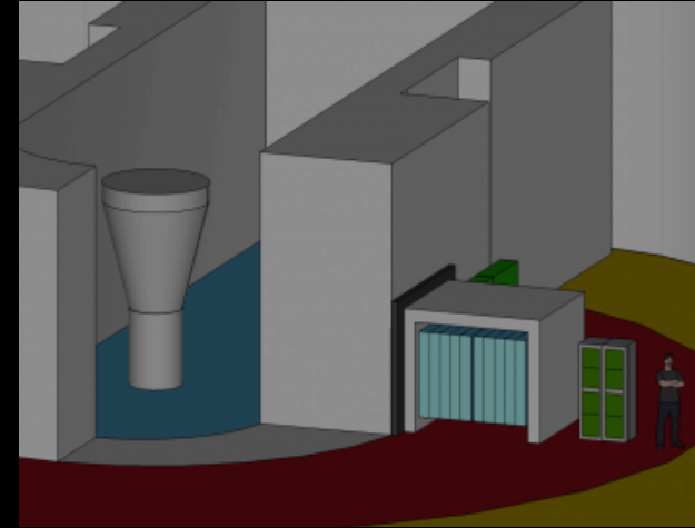
very short baseline neutrino oscillation experiment at BR2 reactor of SCK-CEN (Belgium)
