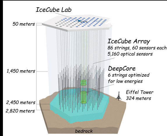
neutrino telescope in the ice on the South Pole
